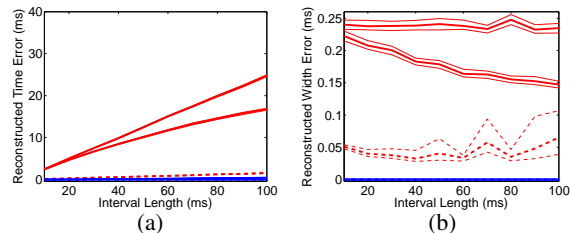
Fig. 5. Signal reconstruction quality versus length of the sampling interval, using a 16-bit ADC at various levels of integration noise. The solid lines show the expected error for low ( \sigma = 0.1 mV) and high ( \sigma = 10 mV) integrator noise. The dashed lines show performance without integration noise. For gAT-1, the lines overlap. Confidence intervals (95%) are based on 100 bootstrapped averages from 10,000 samples.
