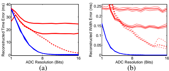
Fig. 4. Signal reconstruction quality as a function of the ADC resolution in bits, in the presence of integrator noise and quantization error. The solid lines show the expected error for a low level of integrator noise ( \sigma = 0.1 mV) and a high level of integrator noise ( \sigma = 10 mV) based on the IVC102 [9]. The dashed lines show performance with no integrator noise, \sigma = 0 mV. For gAT-1, the various lines overlap. Confidence intervals (95%) are based on 100 bootstrapped averages from 10,000 samples.
