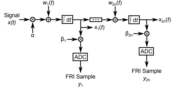
Fig. 2. gAT sampling stage, modeled with integrator noise and quantization error. A square wave input signal x(t) enters a serial bank of noisy integrators and ADCs to obtain the gAT samples y_1, \dots, y_{2n} . Scaling factors \alpha and \beta_i are chosen to maximize performance under worst-case noise-free conditions (see Section 2.2 for details).
