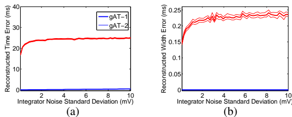
Fig. 3. Using a high-resolution ADC (16 bit), signal reconstruction quality as a function of the integrator noise level \sigma . Sampling interval is 100 ms. Typical simulated spike widths vary between 0.013 ms and 1.12 ms. Confidence intervals (95%) are based on 100 bootstrapped averages from 10,000 samples.
